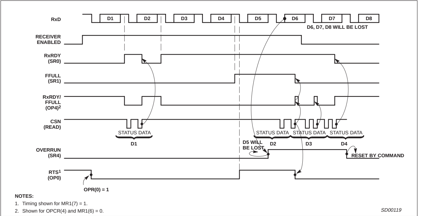
Figure 13. Receive timing
