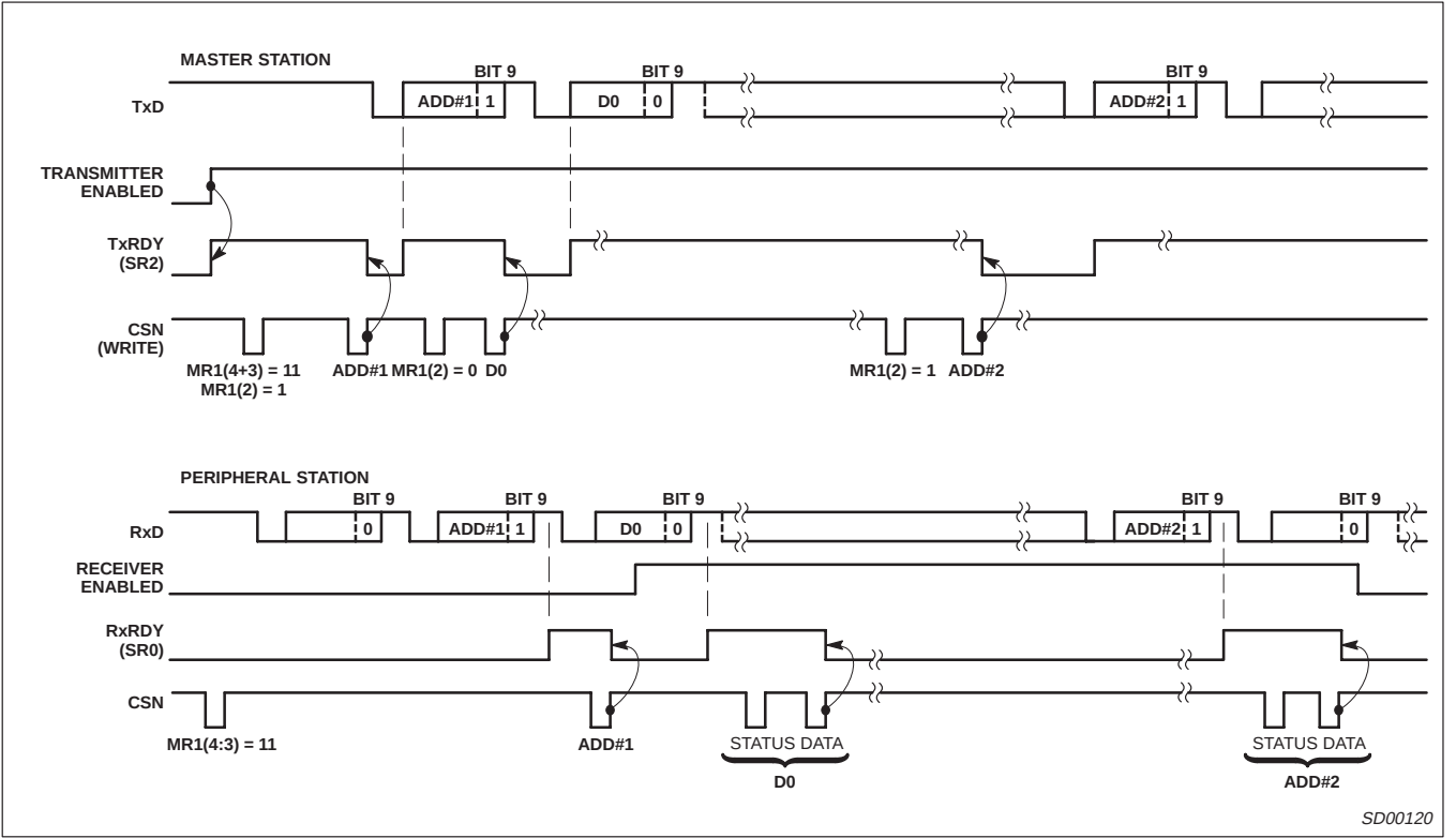
Figure 14. Wake-up mode
