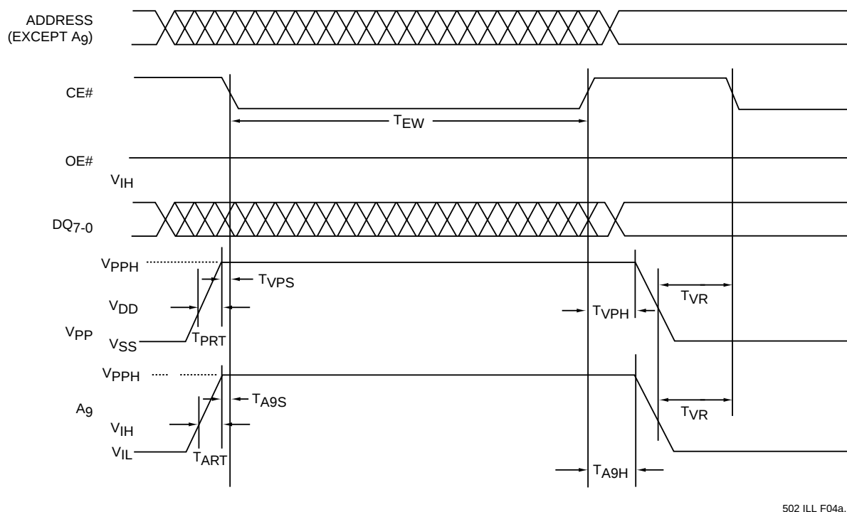
FIGURE 5: CHIP-ERASE TIMING DIAGRAM FOR SST27SF256
