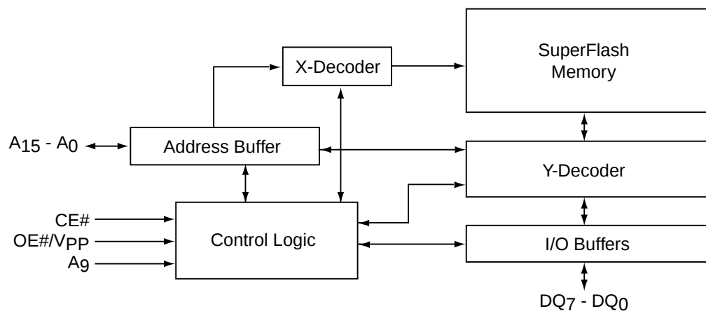
FUNCTIONAL BLOCK DIAGRAM OF THE SST27SF512
