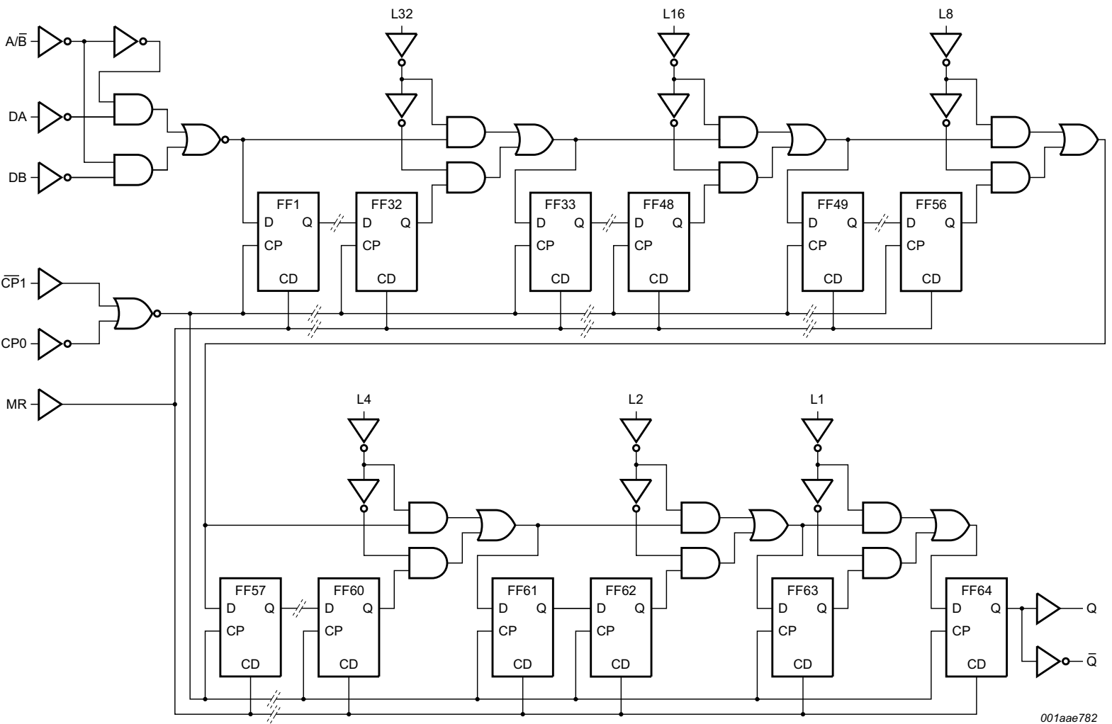
Fig 1. Logic diagram
