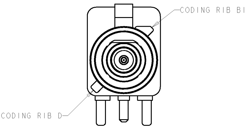
DETAIL G
