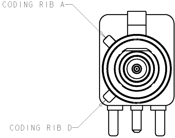
DETAIL D
