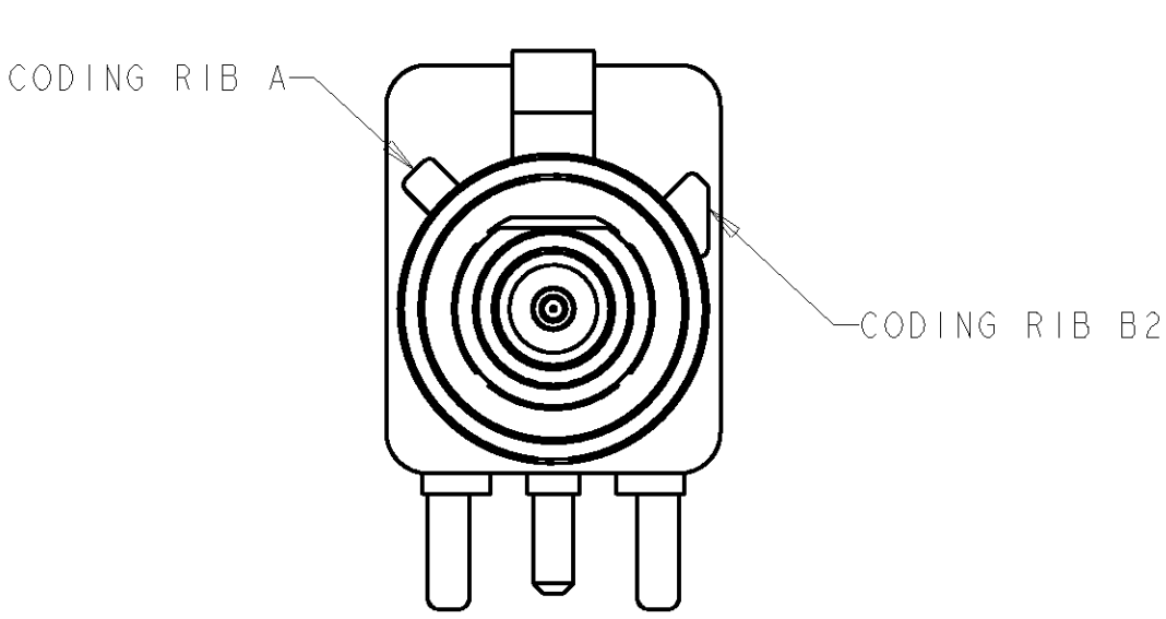
DETAIL B
