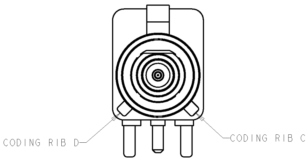
DETAIL K
