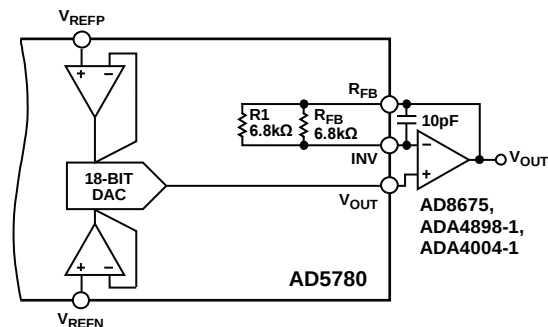
Figure 51. Output Amplifier in Unity Gain with Amplifier Input Bias Current Compensation
