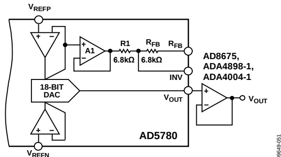
Figure 50. Output Amplifier in Unity-Gain Configuration
