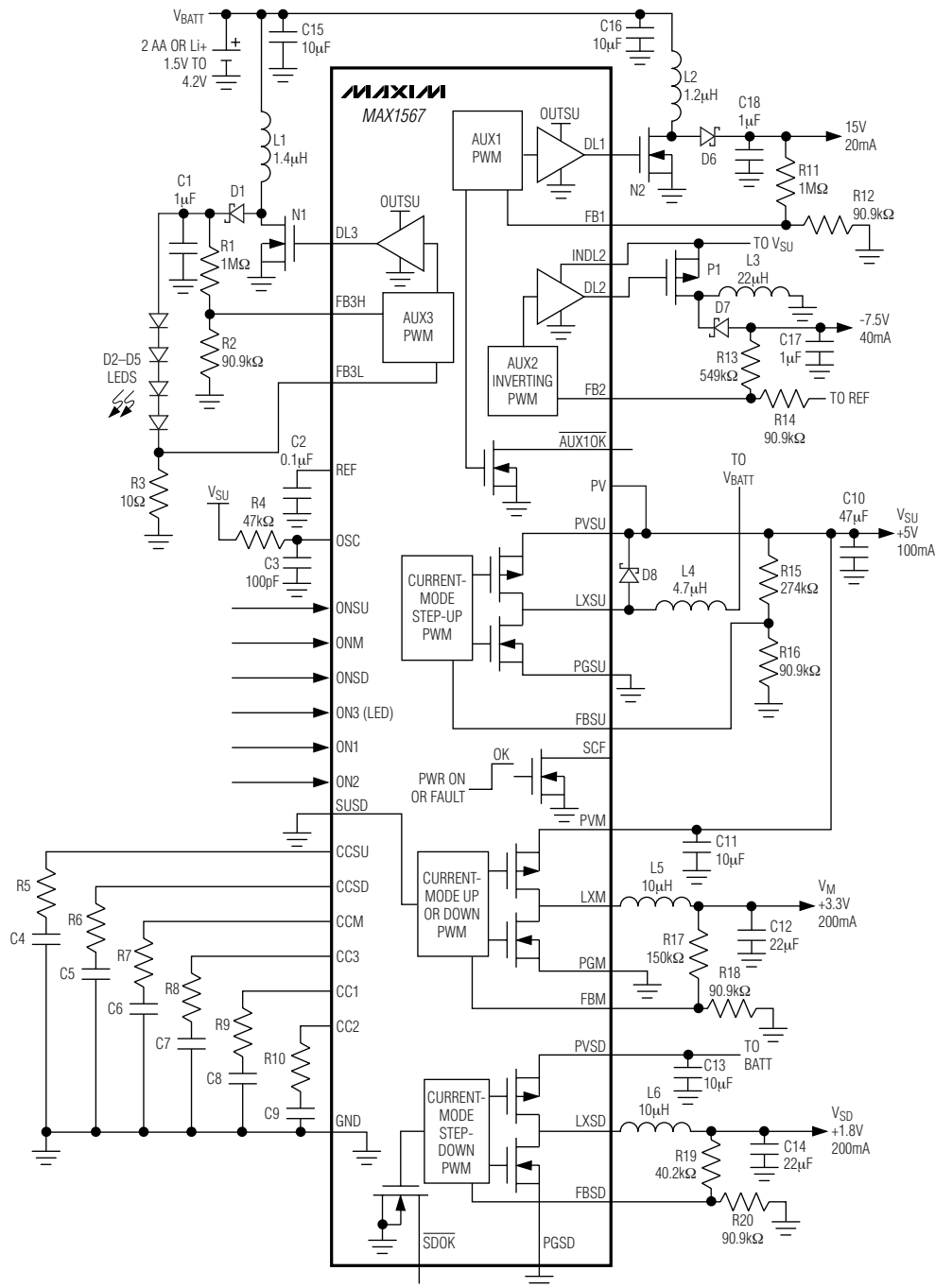
Figure 3. Li+ or Multibattery Input (This power supply accepts inputs from 1.5V to 4.2V, so it can operate from either 2 AA cells or 1 Li+ cell. The 3.3V logic supply and the 1.8V core supply are both stepped down from 5V for true boost-buck operation.)
