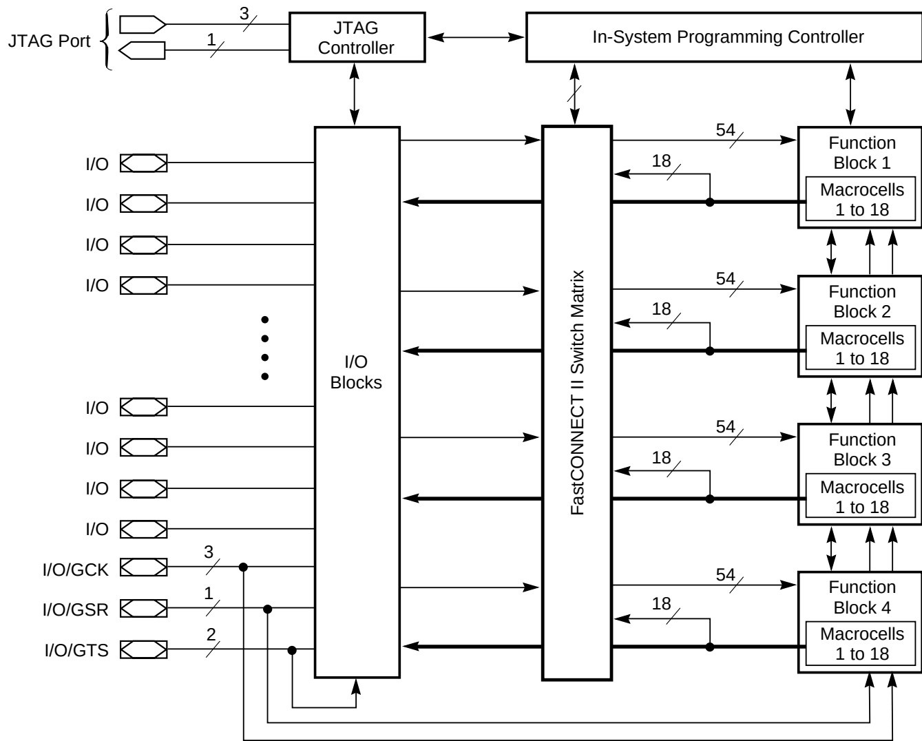
Figure 2: XC9572XV Architecture
