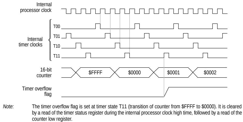
Figure 5-5 Timer state timing diagram for timer overflow
