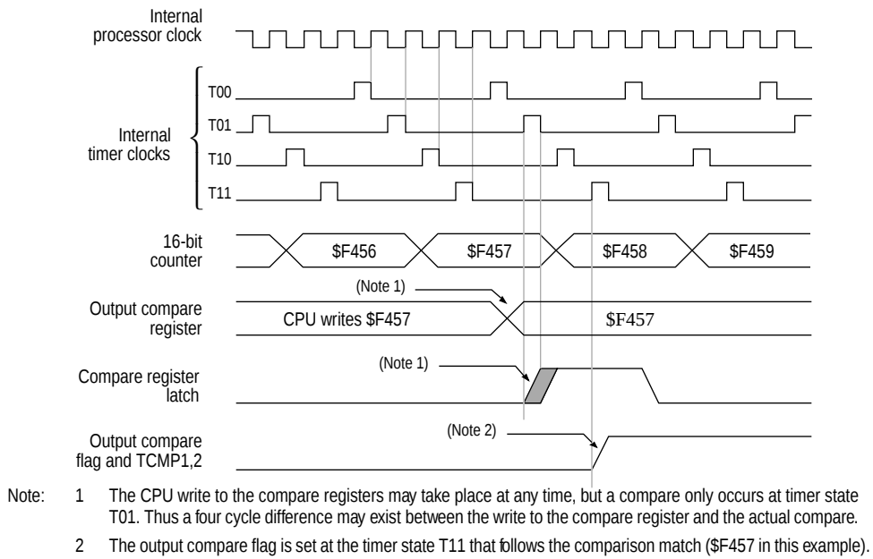
Figure 5-4 Timer state timing diagram for output compare
