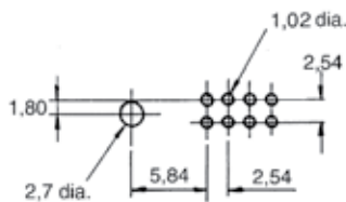
Recommended PCB layouts
