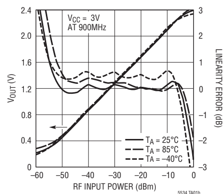
Output Voltage vs RF Input Power
