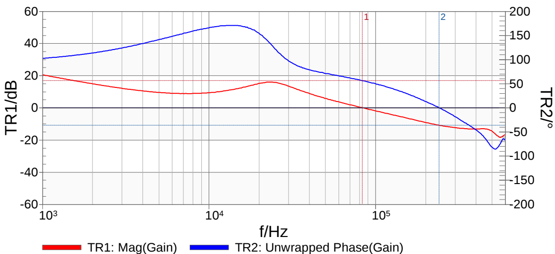
Fig. 12: Bode Plot at 0A load Bandwidth = 83.3kHz, Phase Margin = 56.3^\circ , Gain Margin = 10.8dB
