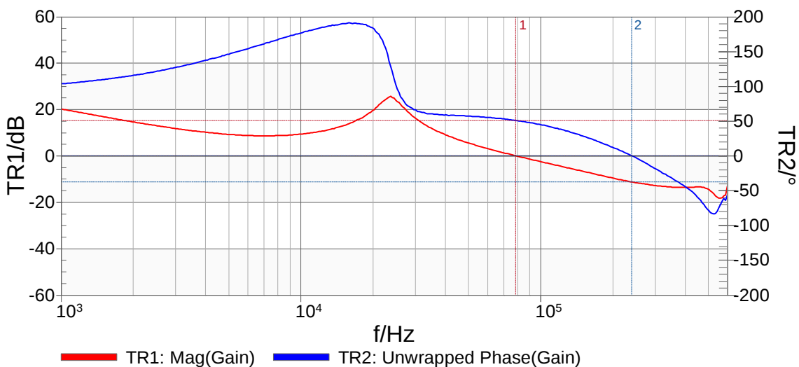
Fig. 13: Bode Plot at 25A load Bandwidth = 78.7kHz, Phase Margin = 50.8^\circ , Gain Margin = 11.3dB
