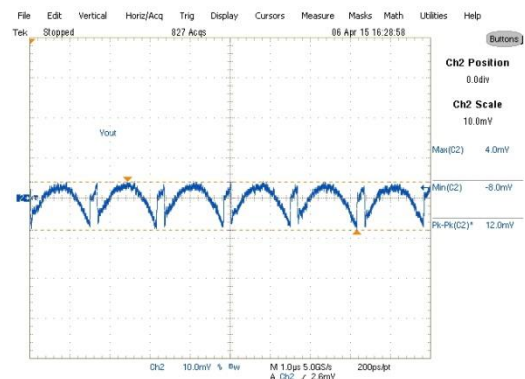
Fig. 7: Output voltage ripple at 25A load Ch 2 : V_{out}
