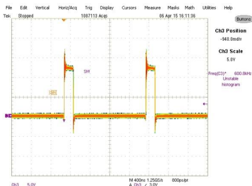
Fig. 6: Inductor node at 25A load Ch 3 :SW node
