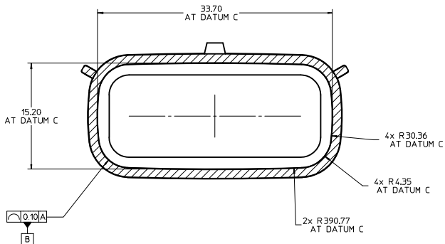
SECTION X-X SCALE 4:1
