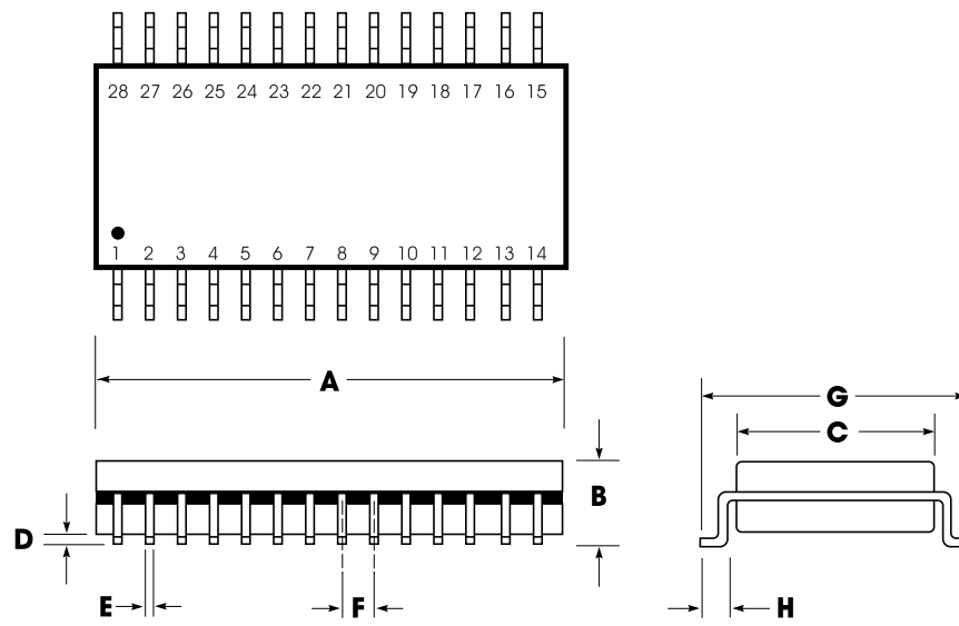
Figure 22: 28-Lead 0.300-Inch Plastic Small Outline Integrated Circuit (SOIC) (S)
