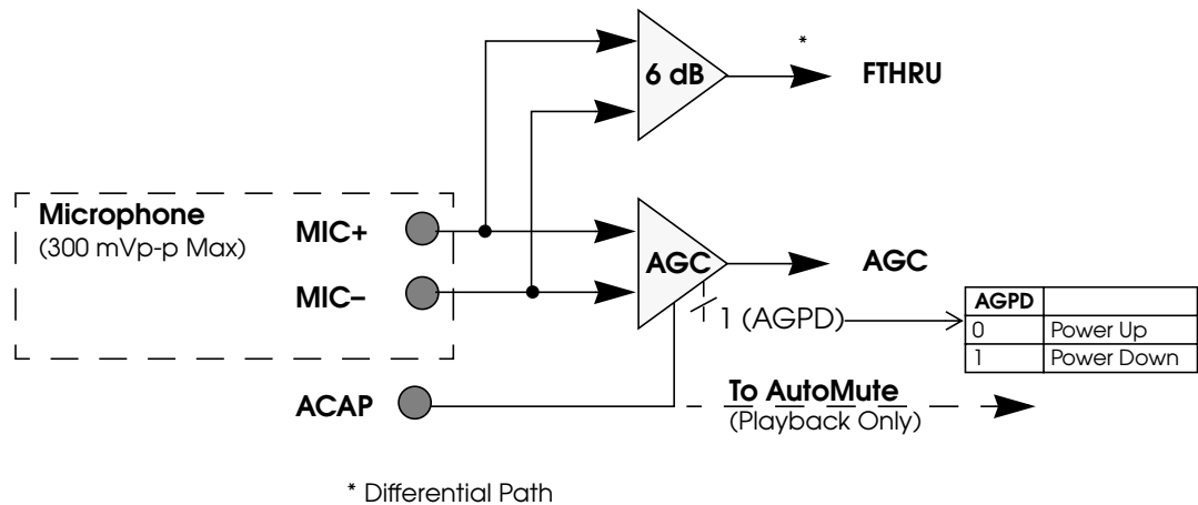
Figure 5: Microphone Amplifier
