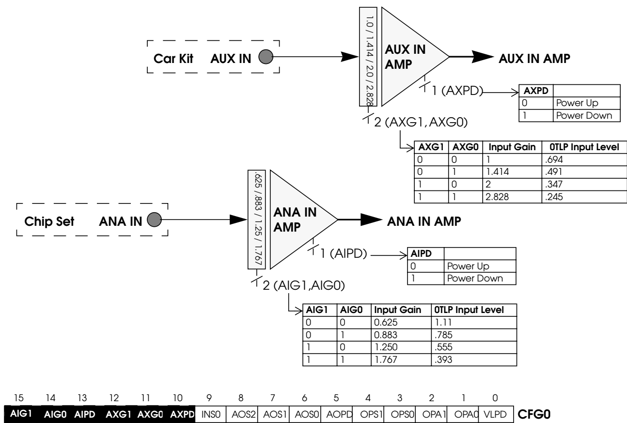
Figure 6: AUX IN and ANA IN
