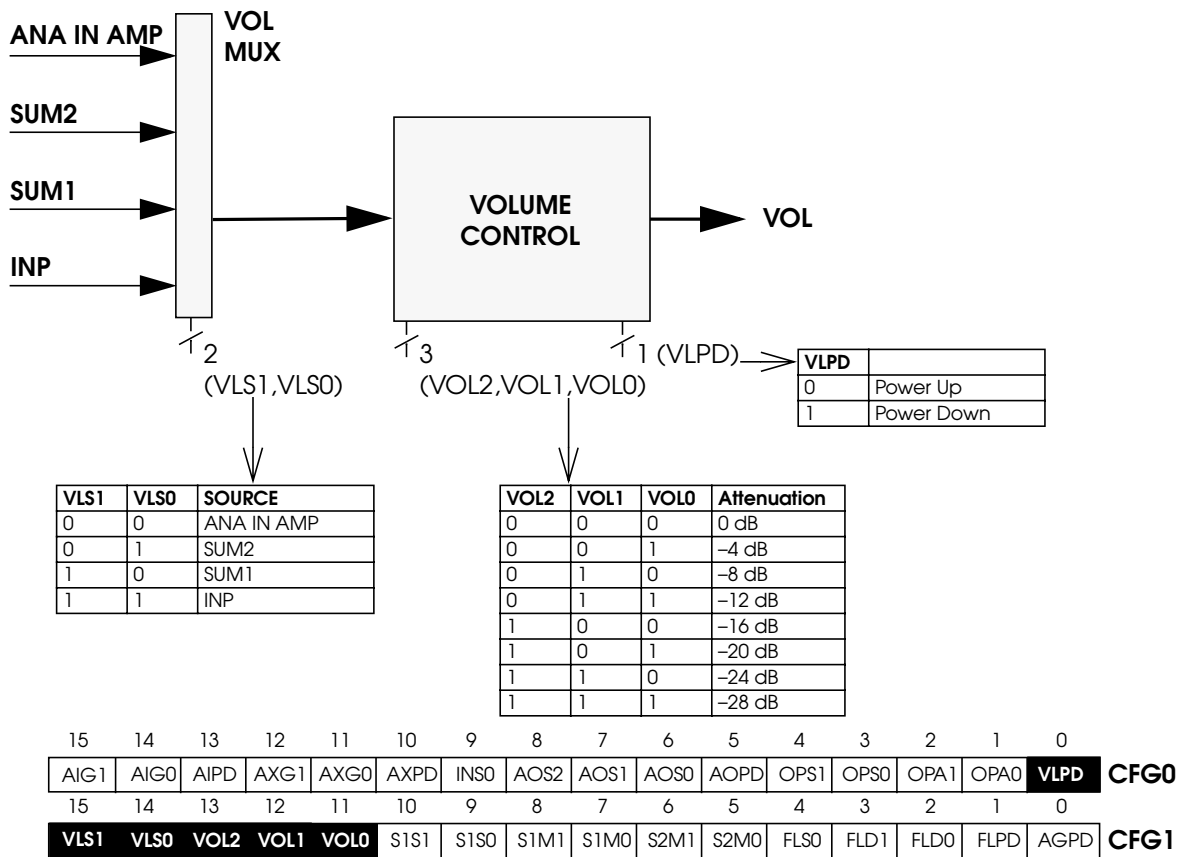
Figure 9: Volume Control
