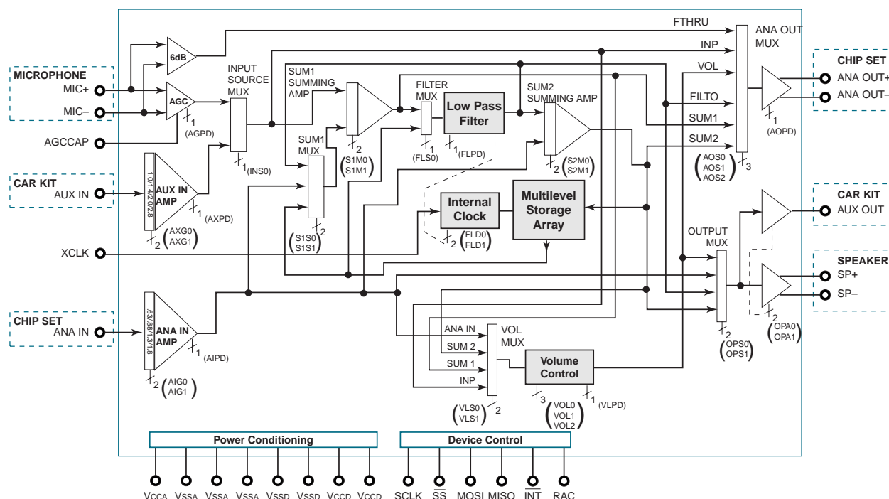
Figure 4-1: ISD5008 Block Diagram
