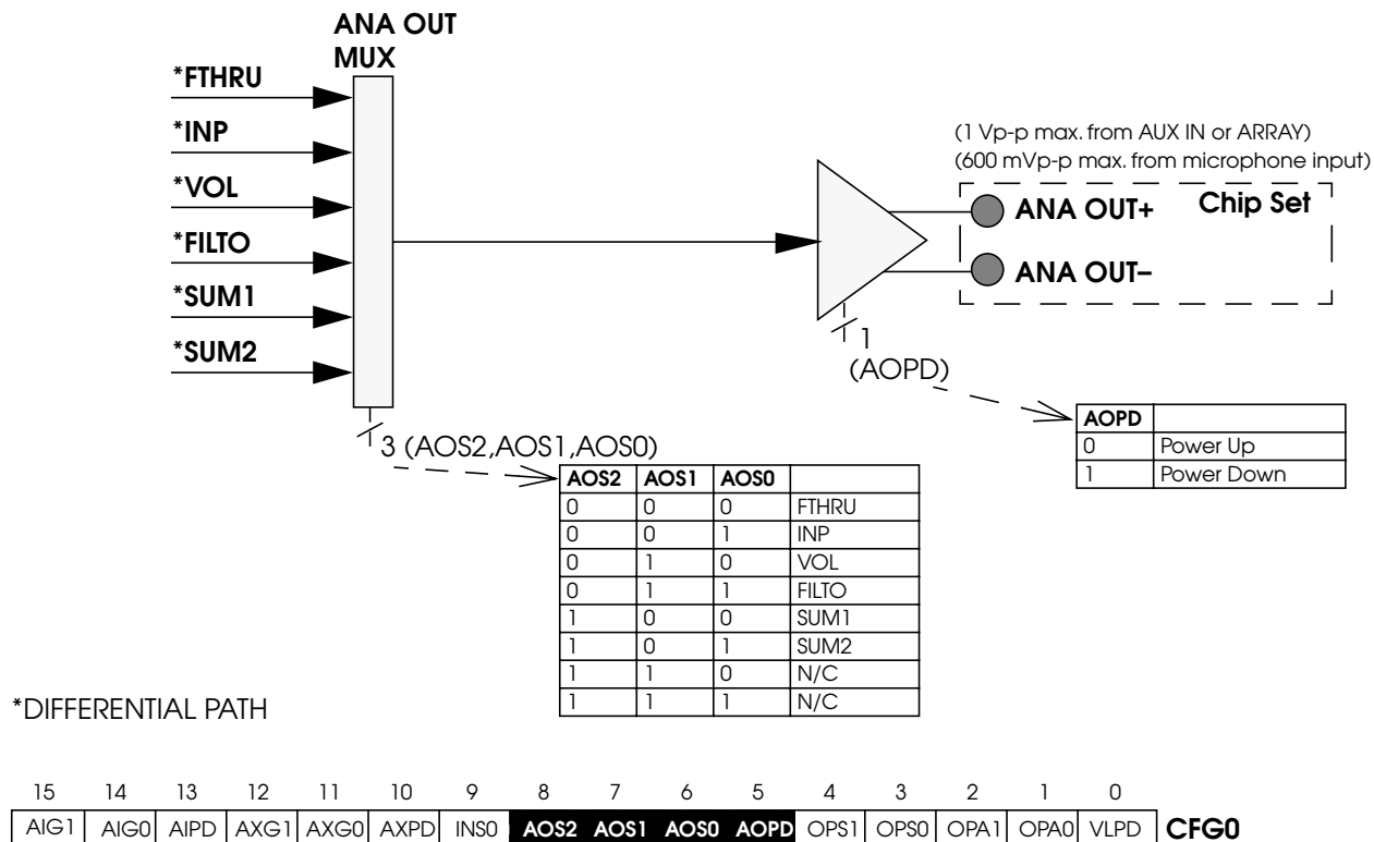
Figure 11: ANA OUT Output
