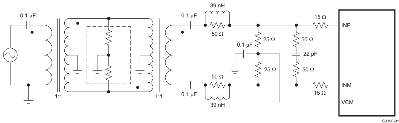
Figure 96. Drive Circuit With Low Bandwidth (for low input frequencies)
