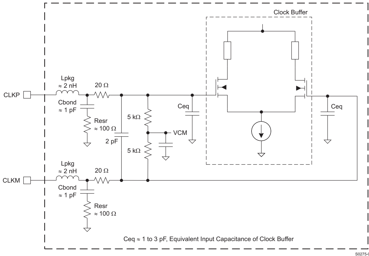
Figure 101. Internal Clock Buffer
