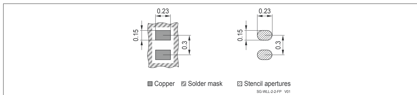
Figure 13 WLL-2-2 footprint (dimension in mm), recommendation for Printed Circuit Board Assembly see [2]
