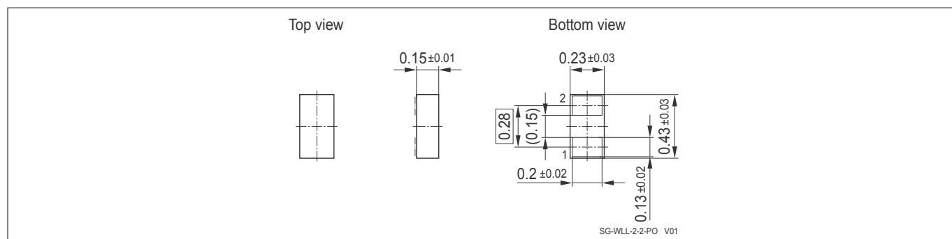
Figure 12 WLL-2-2: package outline (dimension in mm)
