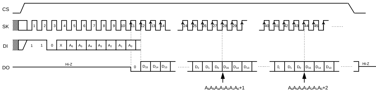
Figure 5 Read Timing (S-93C56A)
