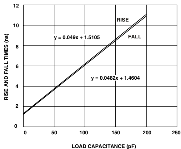
Figure 48. Typical Output Rise/Fall Time (20% to 80%, V_{DD\_EXT} = \text{Min} )
