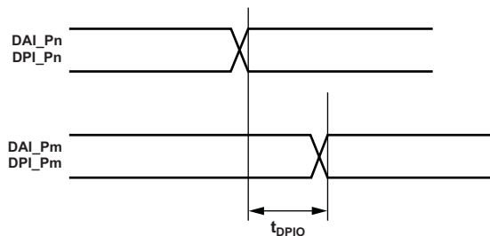
Figure 15. DAI and DPI Pin to Pin Direct Routing
