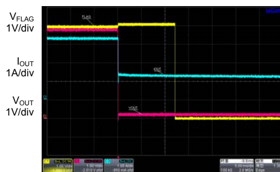
Time 5ms/div
