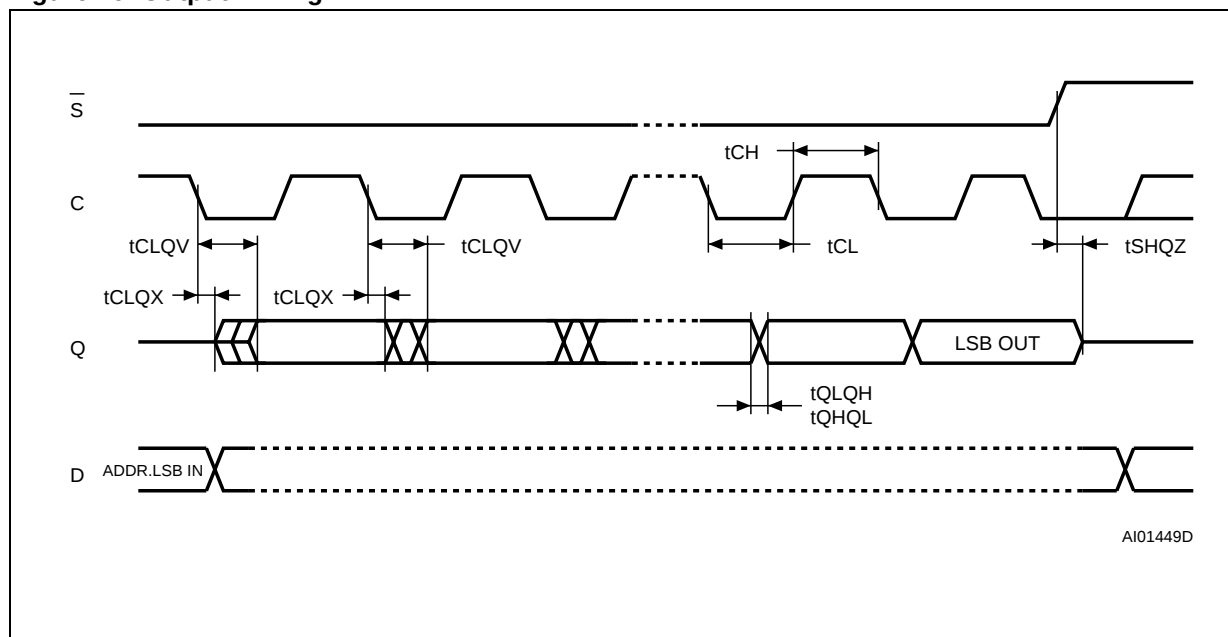
Figure 19. Output Timing
