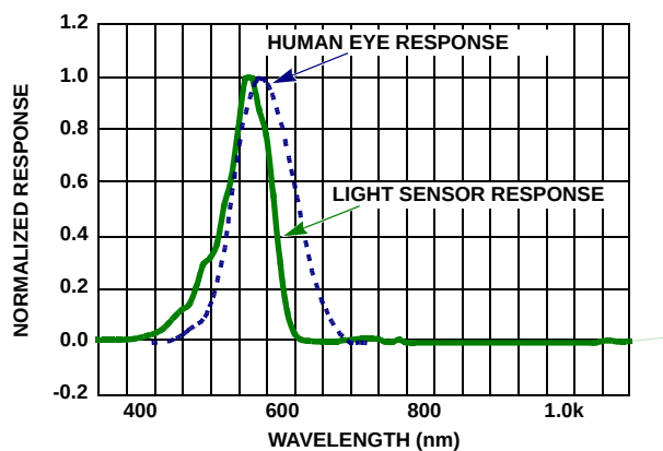
FIGURE 3. SPECTRAL RESPONSE
