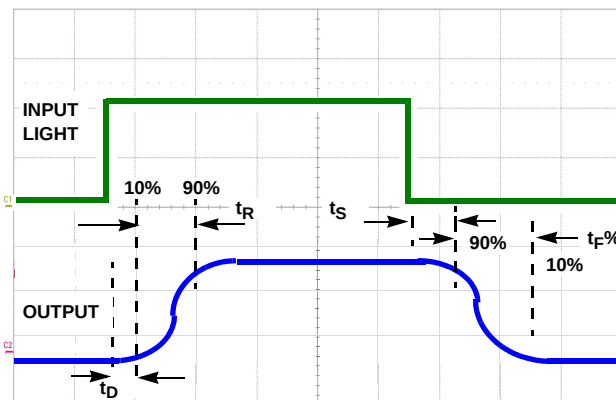
FIGURE 2. TIMING DIAGRAM
