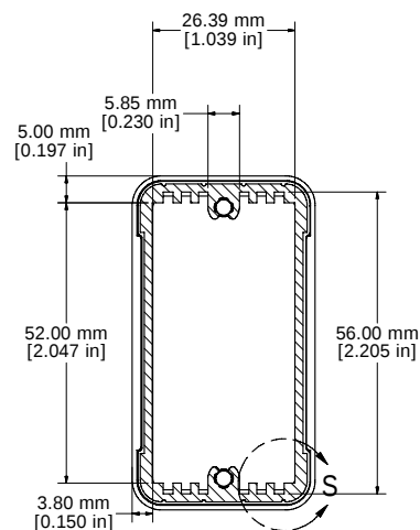
SECTION R-R
