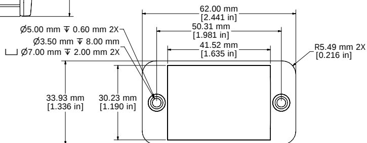
END PANEL - VIEW FROM OUTSIDE
