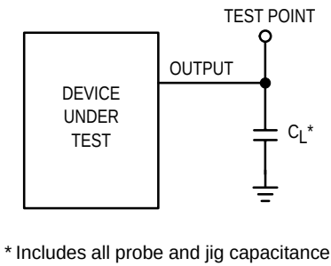
Figure 2. Test Circuit
