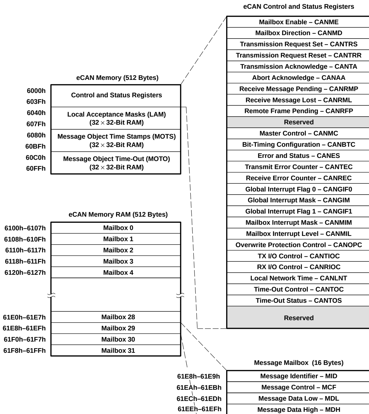
Figure 17. eCAN Memory Map
