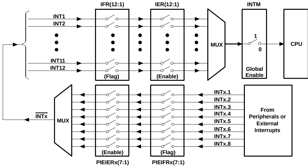
Figure 6. Multiplexing of Interrupts Using the PIE Block
