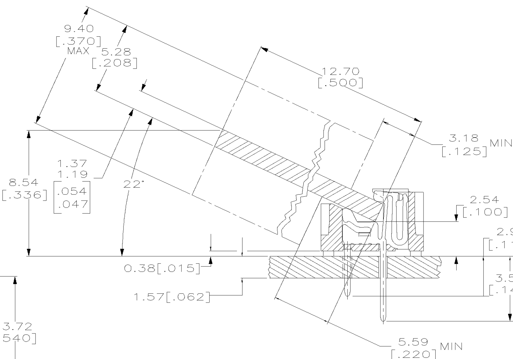
SECTION X-X SCALE 5:1 (BOARD SHOWN FOR REF ONLY)
