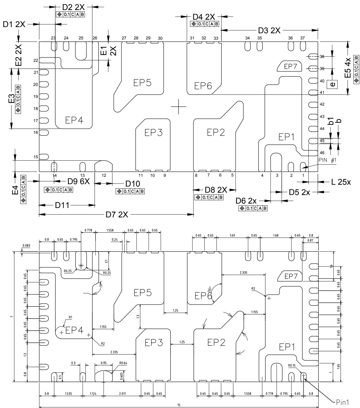
Figure 20. VFQFPN 15 x 7 x 1 mm package dimensions – drawing bottom view
