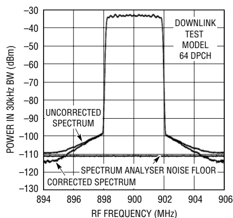
Figure 13. 3-Channel CDMA2000 Spectrum
