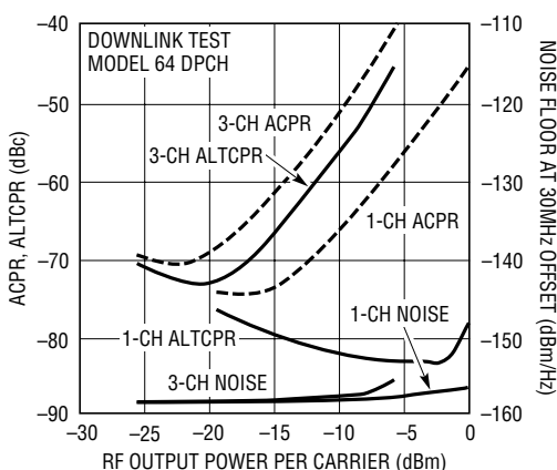
Figure 11. ACPR, ALTCPR and Noise for CDMA2000 Modulation
