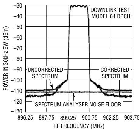
Figure 12. 1-Channel CDMA2000 Spectrum
