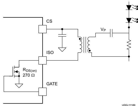
Figure 7. Isolated Current Sense
