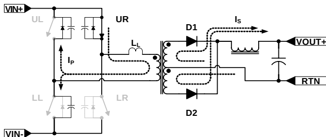
FIGURE 14. UR - UL FREE-WHEELING PERIOD
