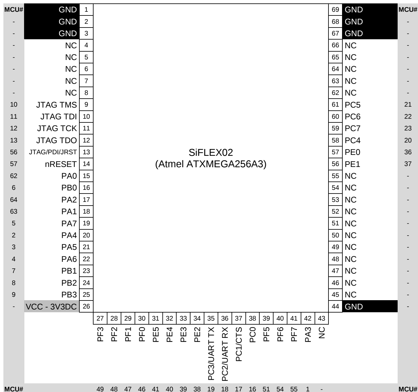
Figure 3 Module Pinout
