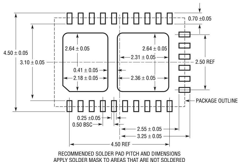
UFE Package 26-Lead Plastic QFN (4mm × 6mm) (Reference LTC DWG # 05-08-1770 Rev A)
