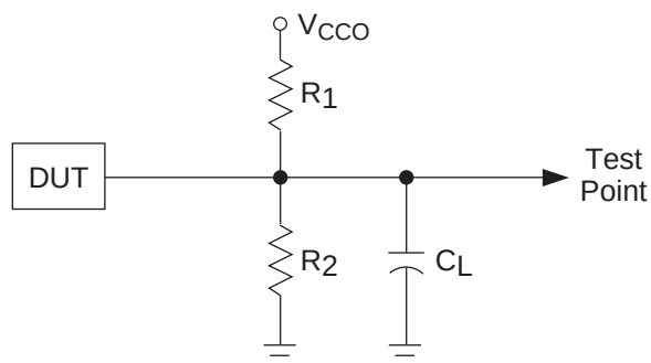
Figure 11. Output Test Load, LVTTTL and LVCMOS Standards
