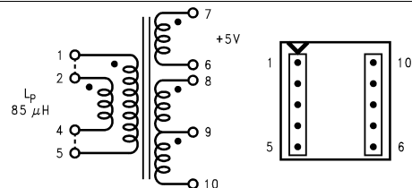
Figure 45. Schott 67140930 (Top View)
