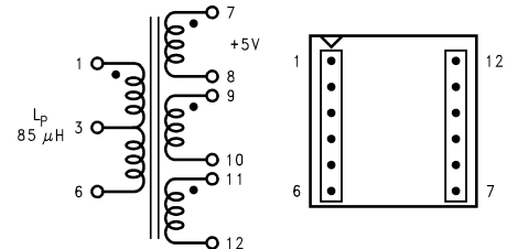
Figure 41. Renco RL-5535 (Top View)
