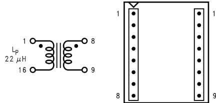
Figure 34. Pulse PE-68411 (Surface Mount) (Top View)
