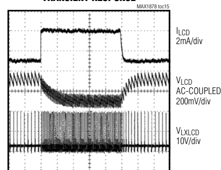
STEP-UP LOAD TRANSIENT RESPONSE
