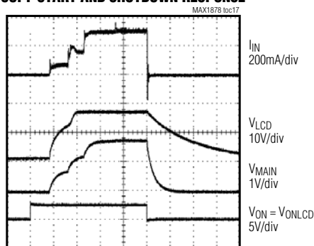
SOFT-START AND SHUTDOWN RESPONSE
