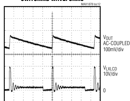
STEP-UP LIGHT-LOAD SWITCHING WAVEFORMS
