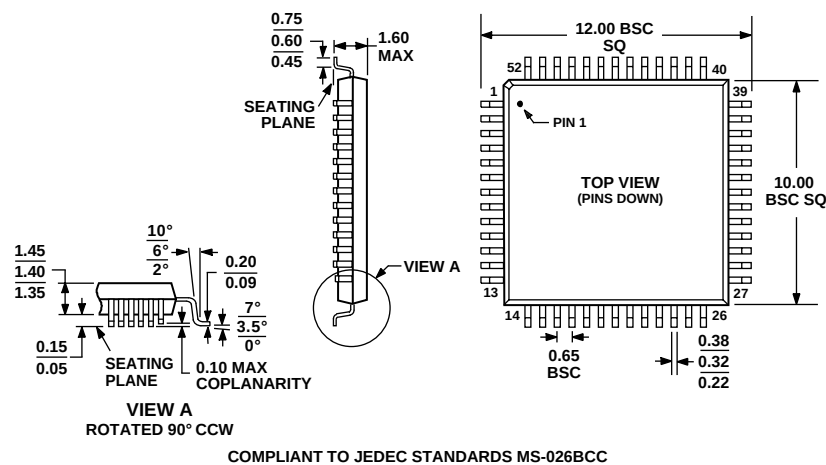
Figure 48. 52-Lead Low Profile Quad Flat Package [LQFP] (ST-52) (Dimensions shown in millimeters)
