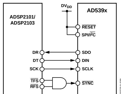
Figure 39. AD539x to ADSP2101/ADSP2103 Interface
