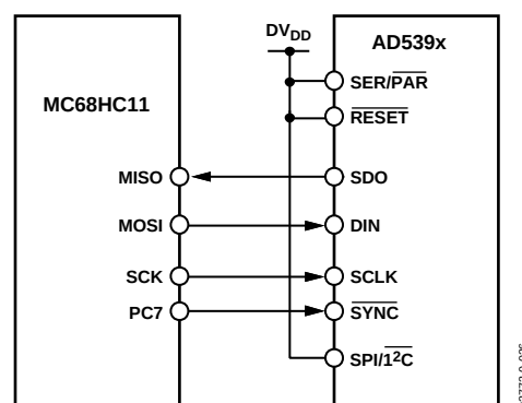
Figure 36. AD539x-MC68HC11 Interface
