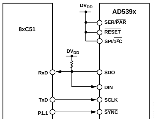
Figure 38. AD539x to 8051 Interface
