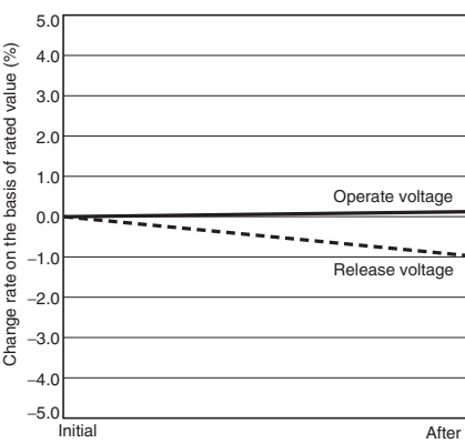
Vibration Resistance
