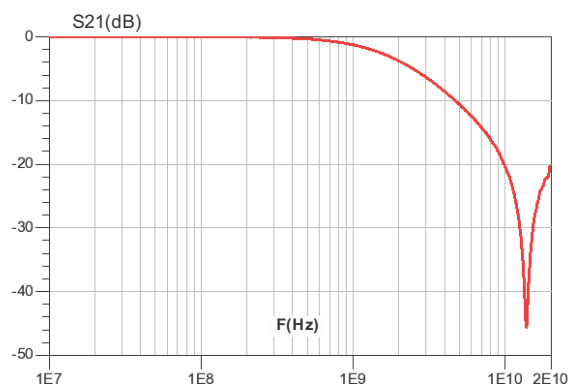
Figure 7. S21 attenuation
