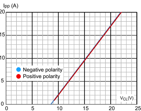
Figure 8. TLP measurementst
