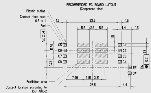
CCM04-1889 PCB Layout
