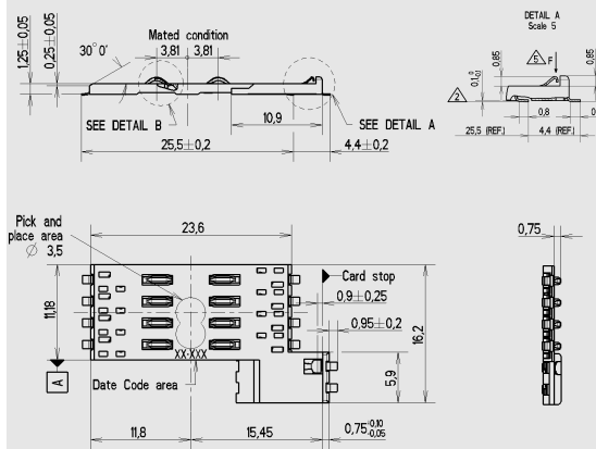
CCM04-1889 2 x 4 contacts + switch
