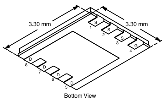
PowerPAK® 1212-8
