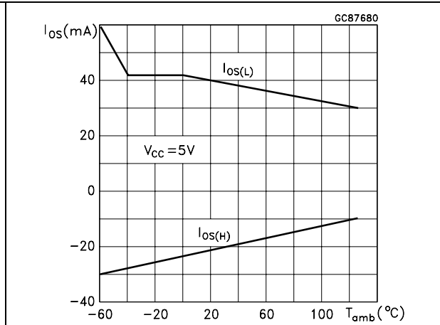
Figure 4. Drive short circuit output current vs temperature
