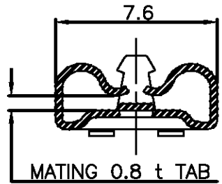
SECT "C"-"C"
