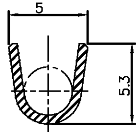
SECT "B"-"B"
