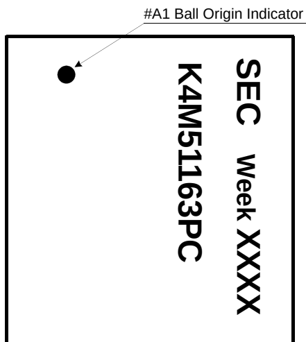
< Top View *2 >
