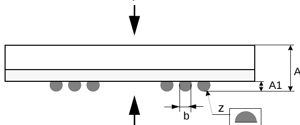
*1: Bottom View
