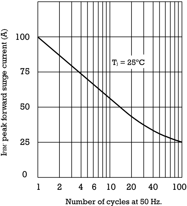
MAXIMUM NON REPETTIVE PEAK FORWARD SURGE CURRENT
