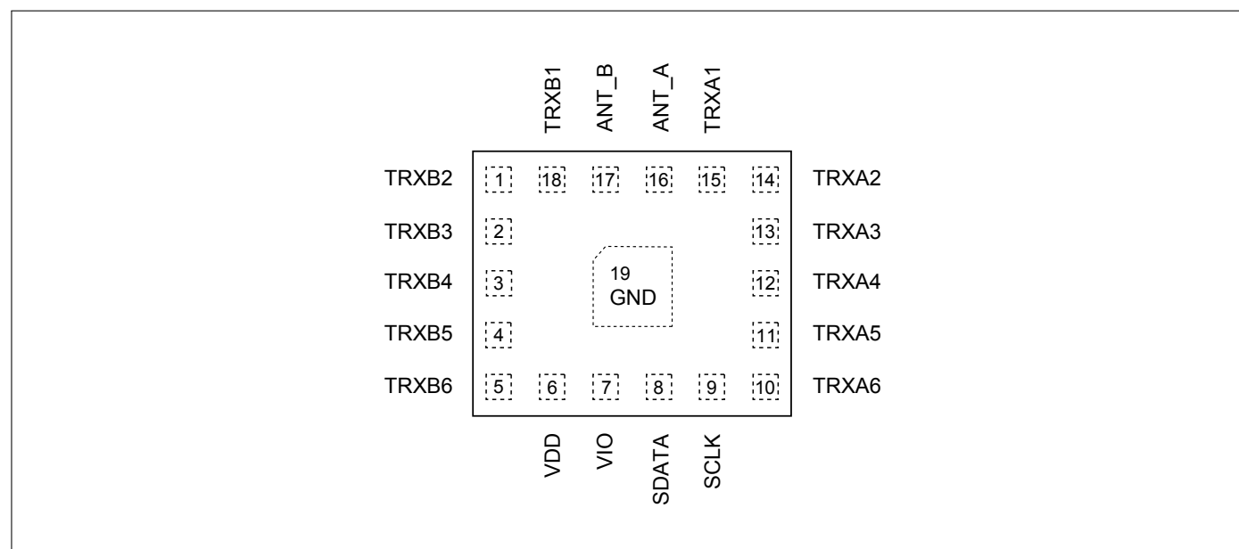
Figure 3: BGSX212MA18 Pin Configuration (top view)
