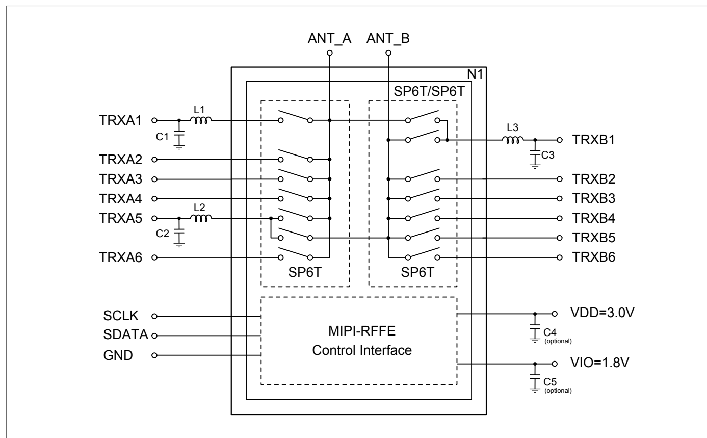
Figure 2: BGSX212MA18 Application Schematic
