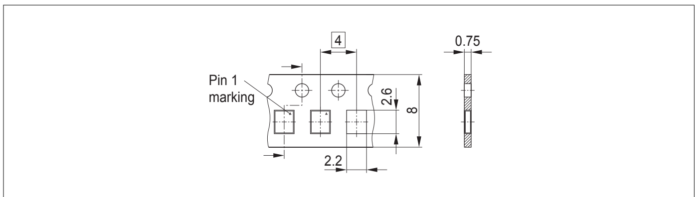
Figure 7: Carrier Tape
