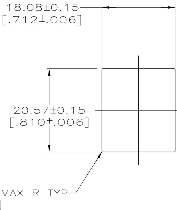
PANEL CUTOUT
