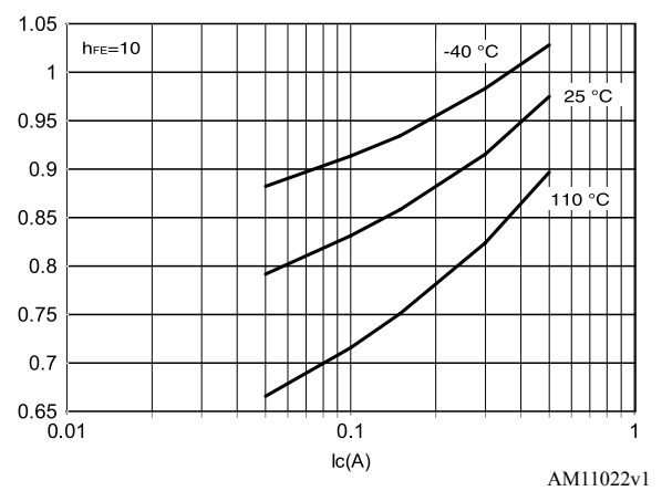
Figure 4. Base emitter saturation voltage ( h_{FE} = 10 )
