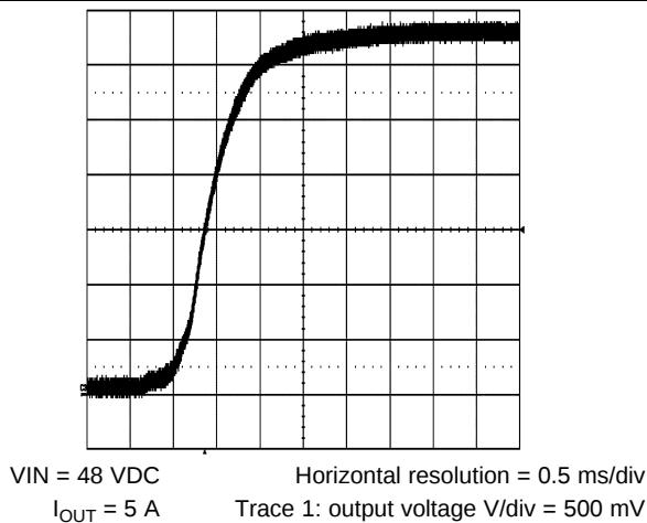
Figure 27. Output Voltage During a Typical Start-Up
