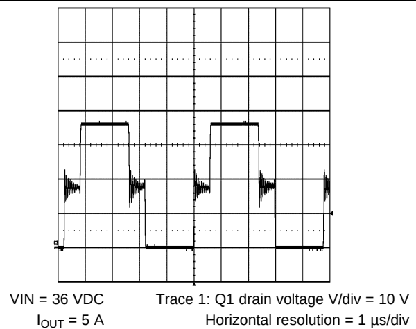
Figure 30. Drain Voltage of Q1 With a 5-A Load
