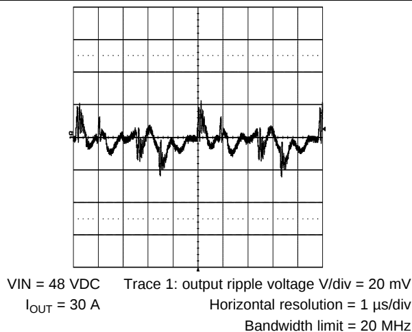
Figure 29. Typical Output Ripple Across the Output Terminals
