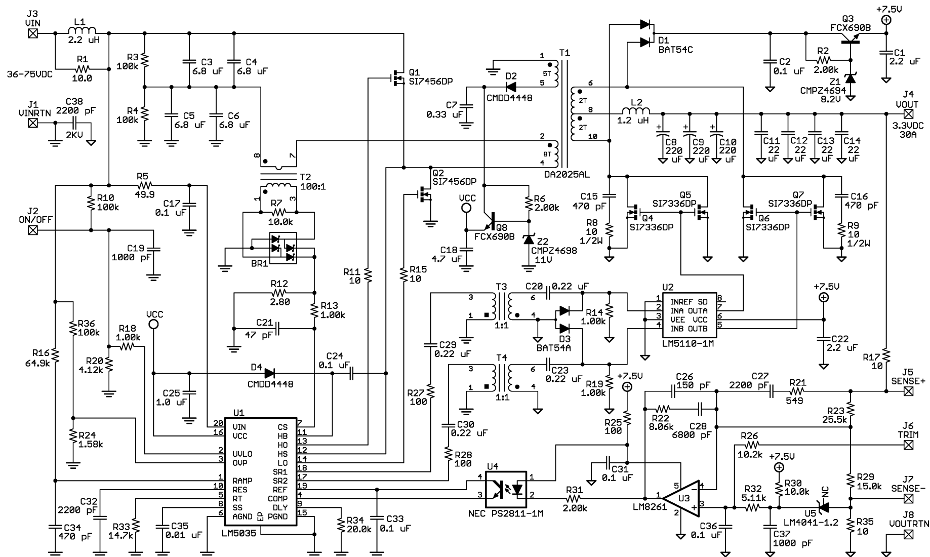
Figure 15. Application Circuit
