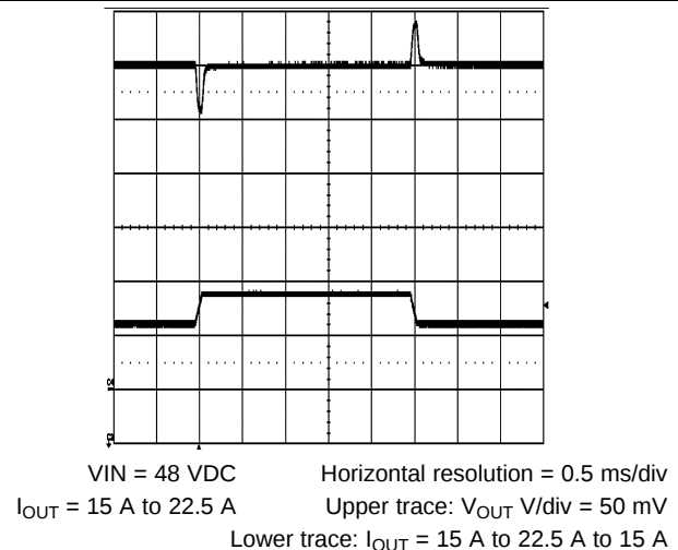
Figure 28. Transient Response for a Load Change From 15 A to 22.5 A
