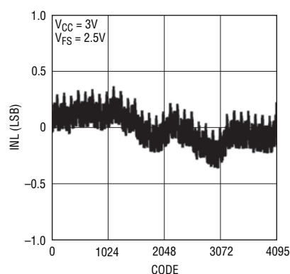
Integral Nonlinearity (LTC2631A-LM12)
