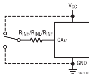
Test Circuit 2
