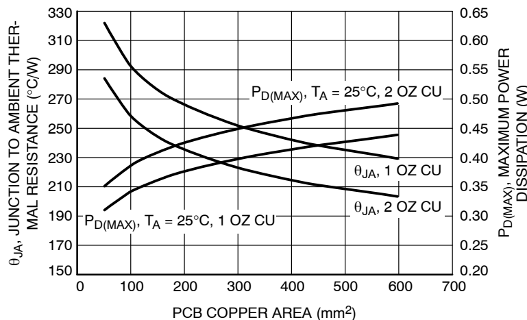
Figure 62. \theta_{JA} and P_{D(\text{MAX})} vs. Copper Area (TSOP5)
