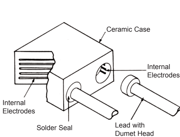
Radial C 3 - One Lead Removed
