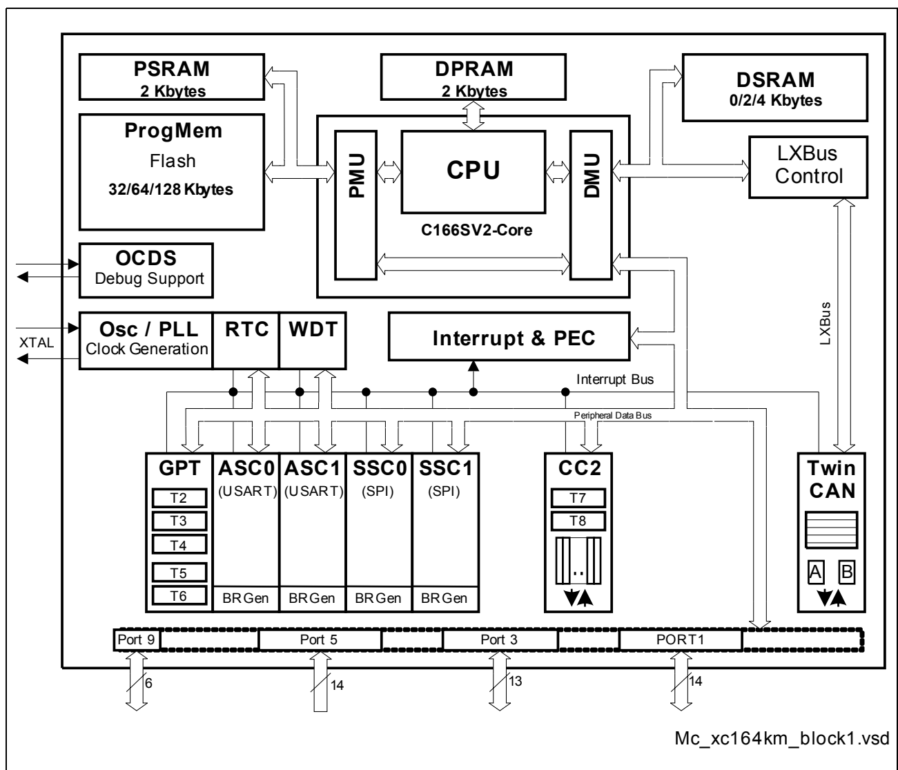
Figure 3 Block Diagram
